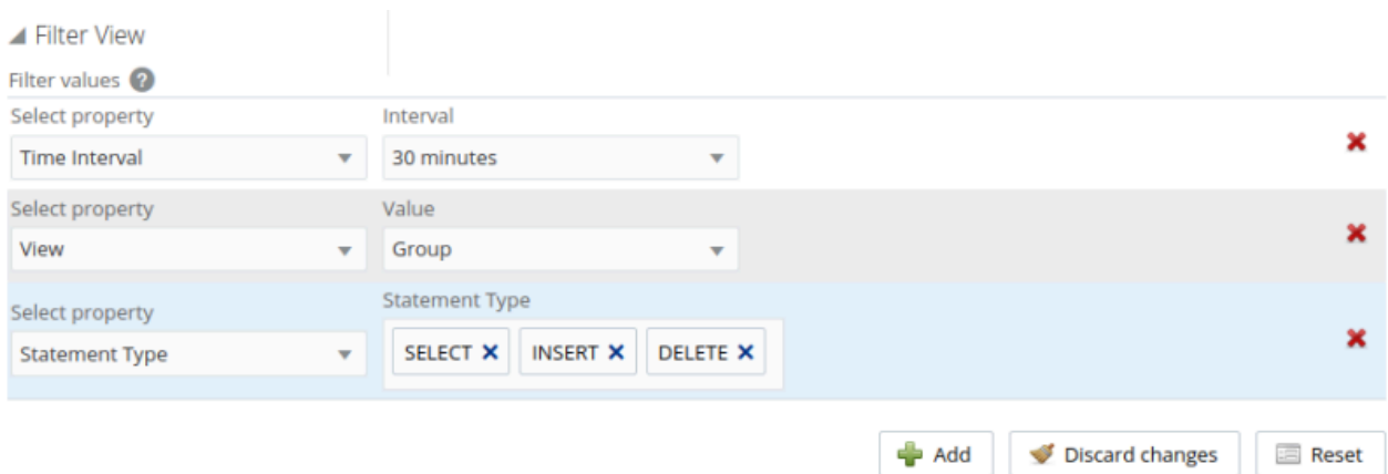
Figure 32.9 Filter View
